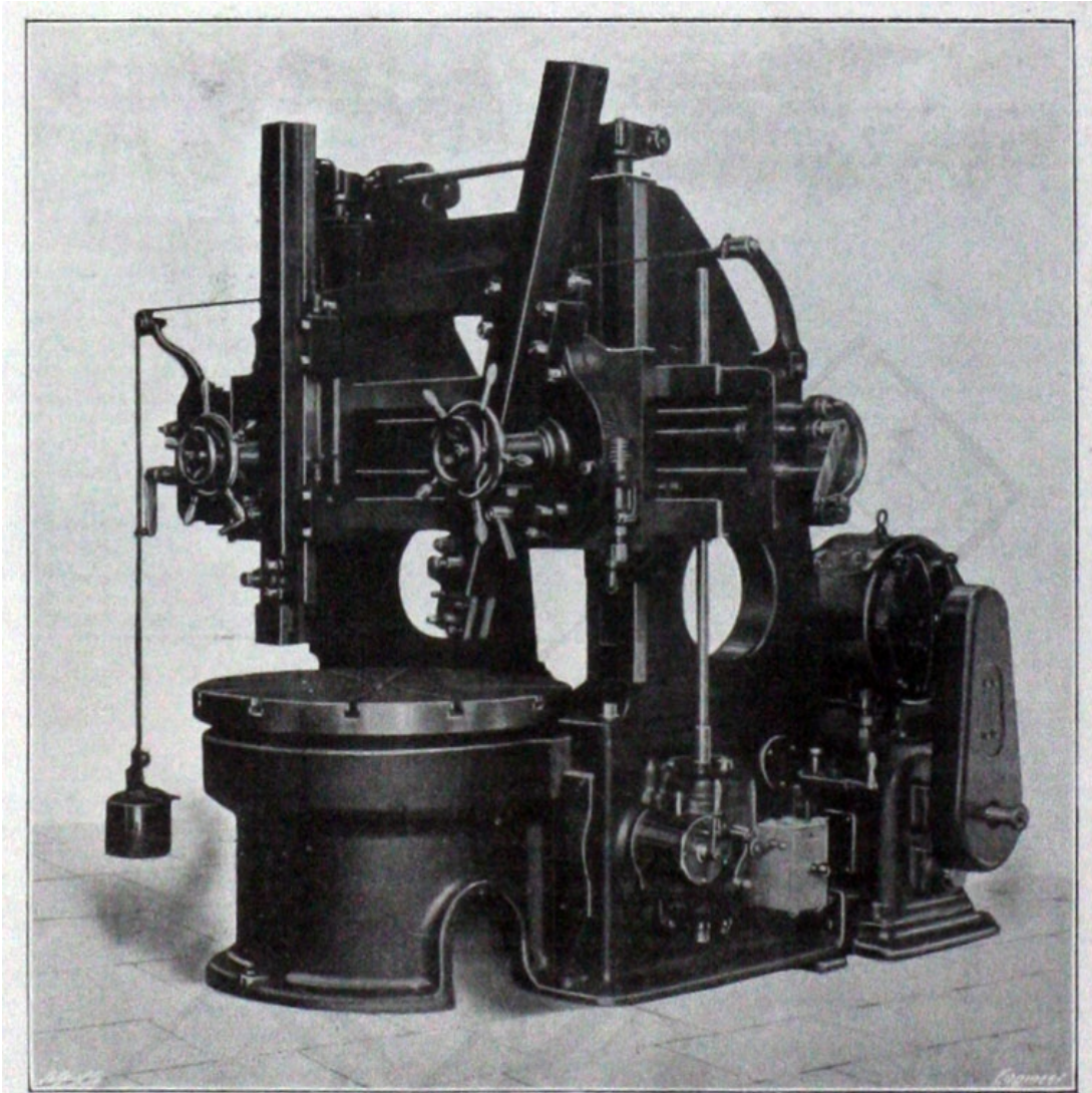
Fig. 42—48-INCH BORING AND TURNING MILL
